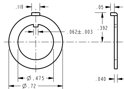
SCREW, LOCKWASHER (PART NO. TL-10090) BRASS-TIN PLATED
