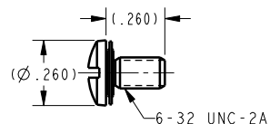
SCREW, LOCKWASHER (PART NO. TL-10090) BRASS-TIN PLATED
