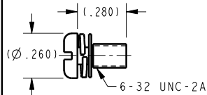
SCREW, LOCKWASHER (PART NO. TL-10122) STEEL-TIN PLATED
