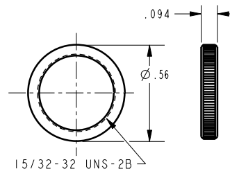
15/32-32 UNS-2B KNURLED NUT (PART NO. TS-10390) NICKEL PLATE BRIGHT BRASS
