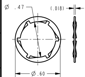
LOCKWASHER (PART NO. TS-10398) CAD PLATE-C.R. STEEL
