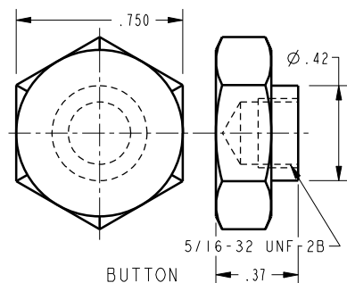
5/16-32 UNF-2B BUTTON (PART NO. TL-10547) BRASS-NICKEL PLATE
